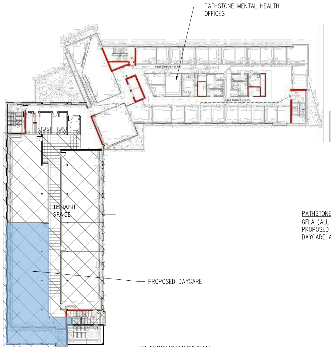
EX. SECOND FLOOR PLAN
